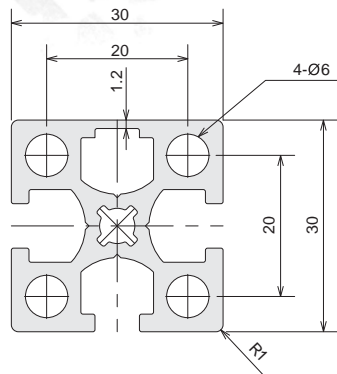
CAD Drawing
