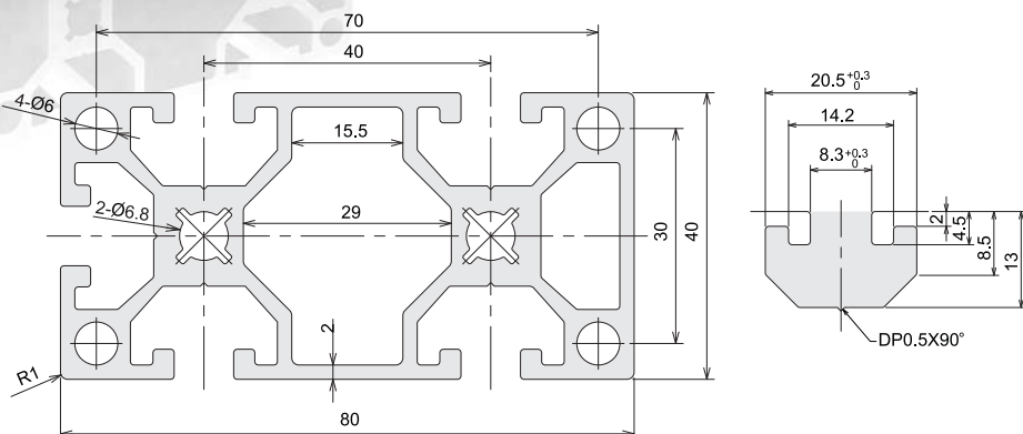
CAD Drawing
