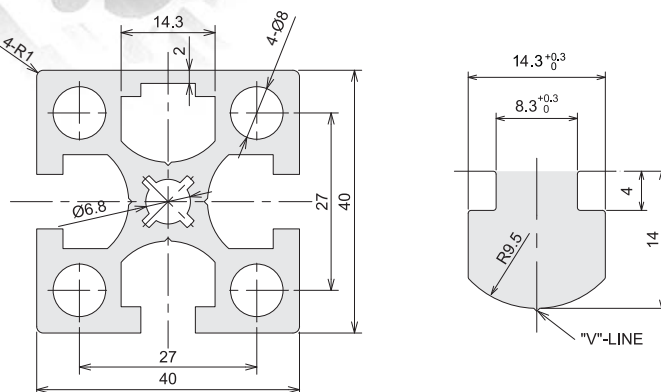
CAD Drawing
