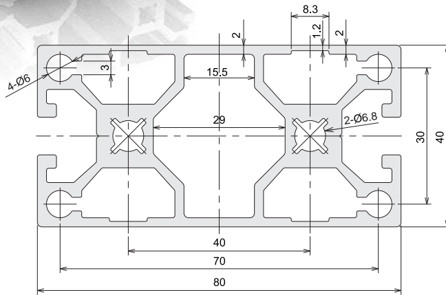
CAD Drawing
