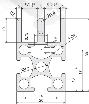
CAD Drawing
