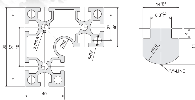
CAD Drawing
