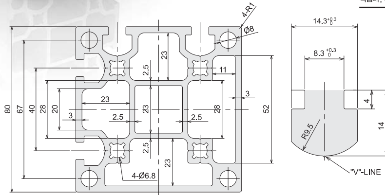
CAD Drawing
