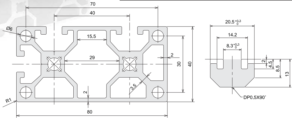
CAD Drawing
