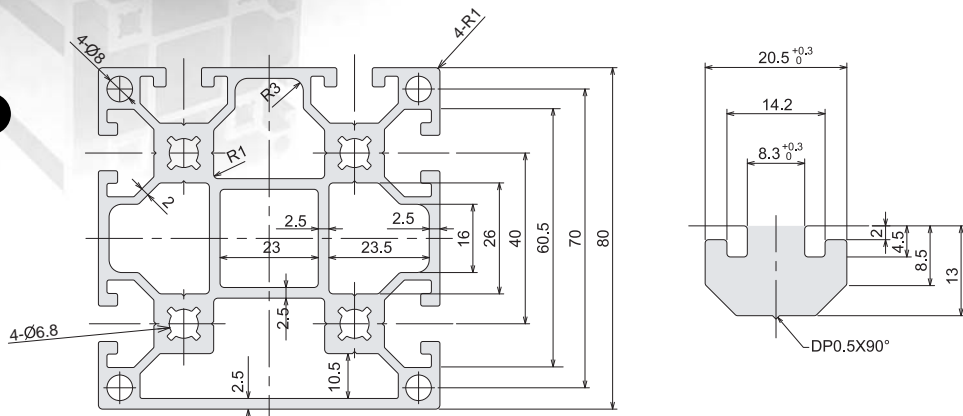
CAD Drawing
