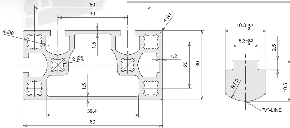
CAD Drawing
