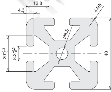
CAD Drawing
