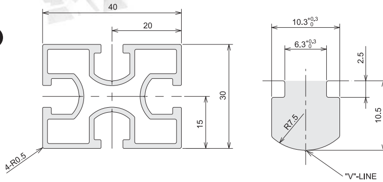
CAD Drawing
