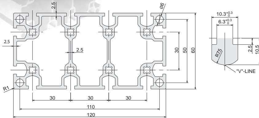
CAD Drawing
