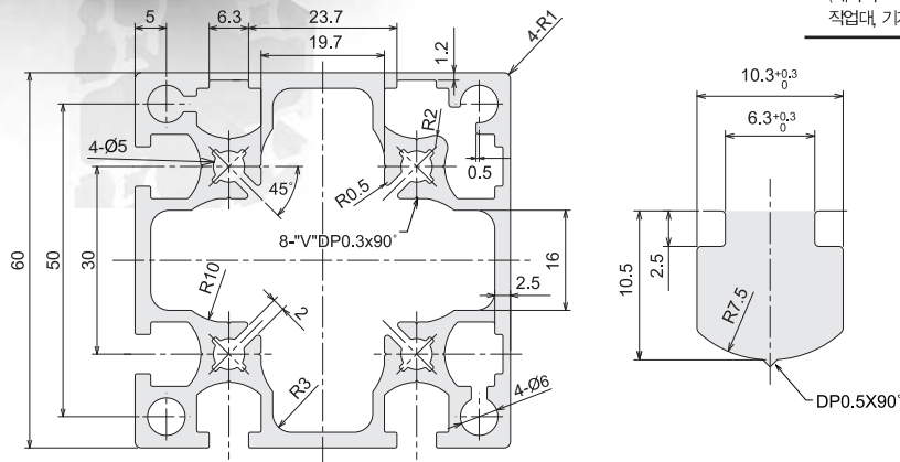
CAD Drawing
