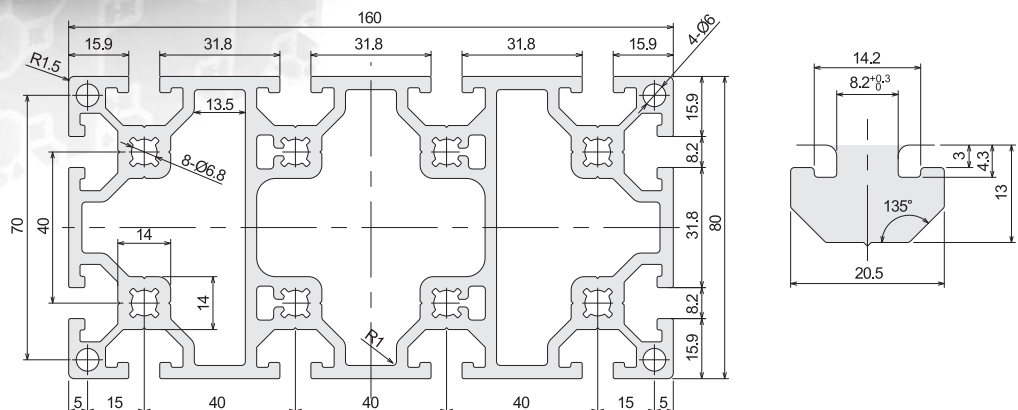
CAD Drawing
