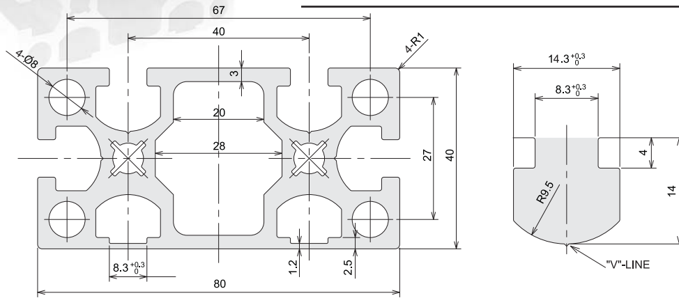
CAD Drawing
