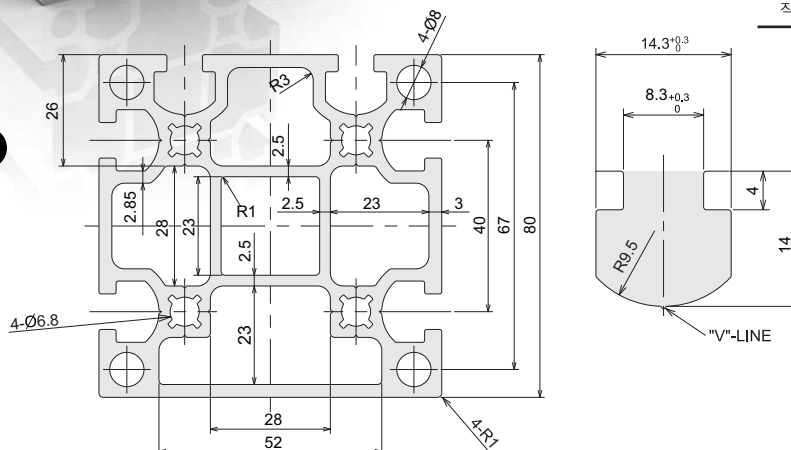
CAD Drawing
