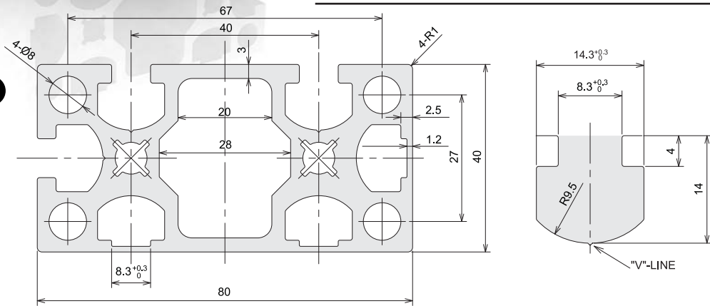
CAD Drawing
