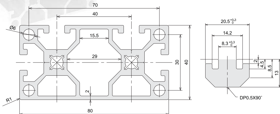
CAD Drawing
