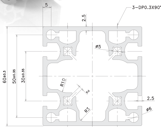
CAD Drawing
